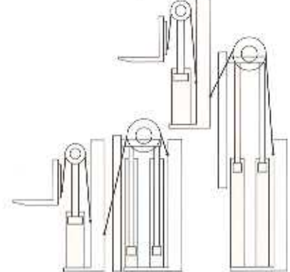
3stage Full Free Mast
