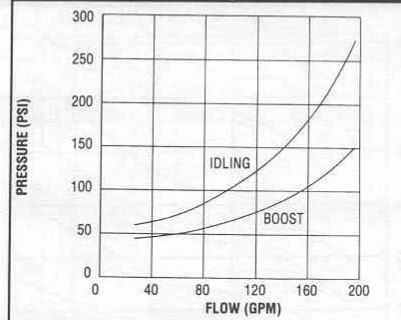
Idling Pressure and Boost Pressure Requirement
