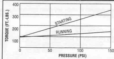
Torque Requirement When Free Wheeling
