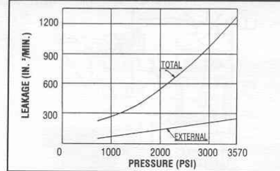
Static Leakage
